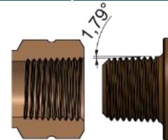
BSPT ISO 7/1 (DIN 3852-2 C)
