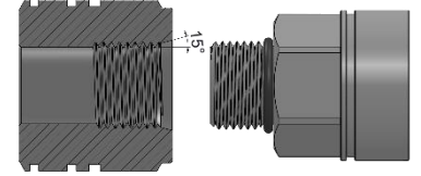
SAE J1926 / ISO 11926 (ORB)
